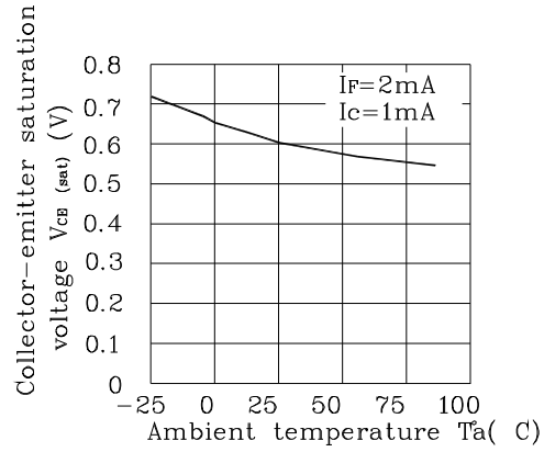
Fig.5 Collector-emitter Saturation Voltage vs. Ambient Temperature
