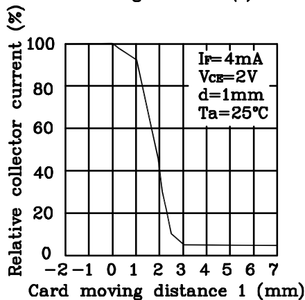
Fig.8 Relative Collector Current vs. Card Moving Distance(1)
