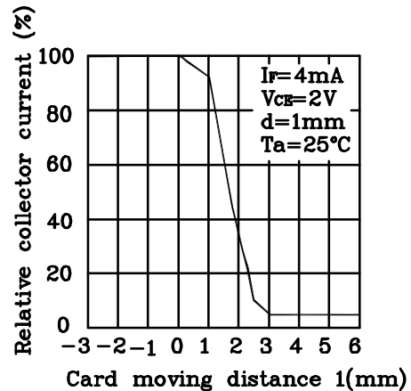
Fig.9 Relative Collector Current vs. Card Moving Distance(2)
